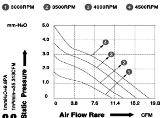
JAMICON FAN PERFORMANCE CURVES
