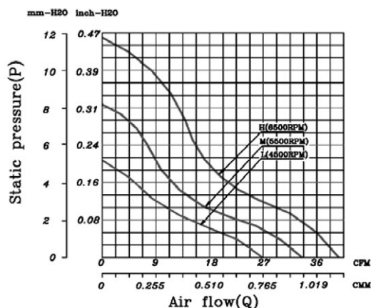
JAMICON FAN PERFORMANCE CURVES
