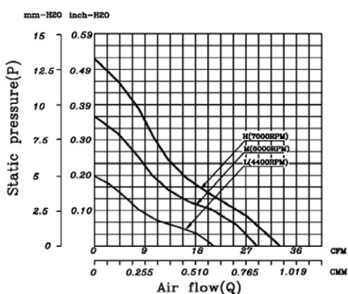
JAMICON FAN PERFORMANCE CURVES
