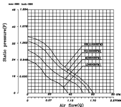
JAMICON FAN PERFORMANCE CURVES
