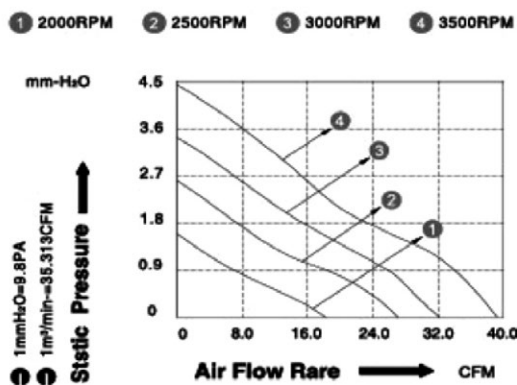
JAMICON FAN PERFORMANCE CURVES
