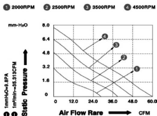
JAMICON FAN PERFORMANCE CURVES
